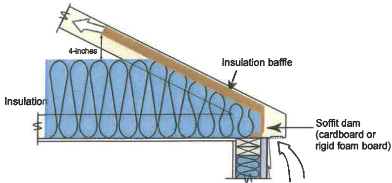
Standard Truss with tapered insulation depth
