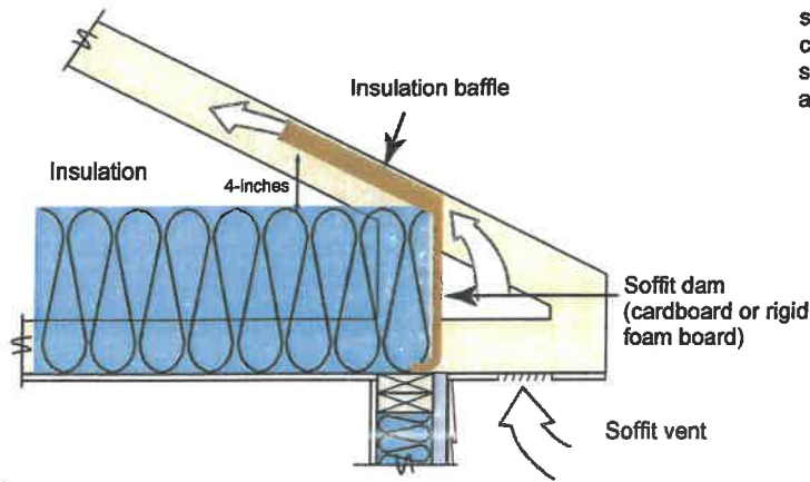
Energy Truss with full height insulation (recommended)
